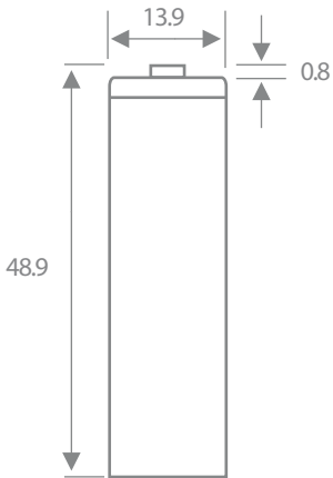
Typical dimensions (mm). Without tube.
